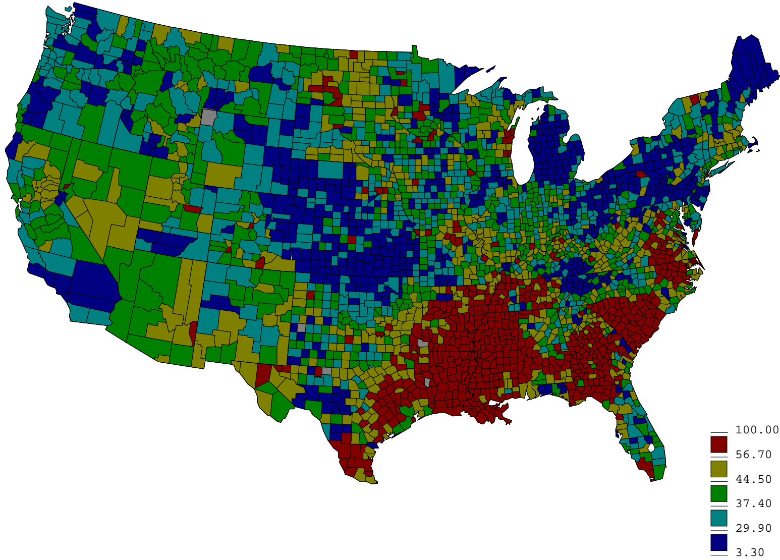
Map Title: e928_1 Percent of votes for Democratic candidate (Alfred E. Smith)
