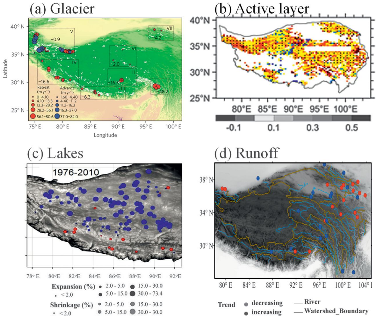
FIG. 3. (a) Observed changes in glacier ( \text{m yr}^{-1} ; from Yao et al. 2012b), (b) simulated changes in active layer thickness during 1981–2010 ( \text{m decade}^{-1} ; from Guo and Wang 2013), (c) observed changes in lake areas during 1976–2010 (from Lei et al. 2014), and (d) runoff change based on hydrological station data (modified from Cuo et al. 2014).
