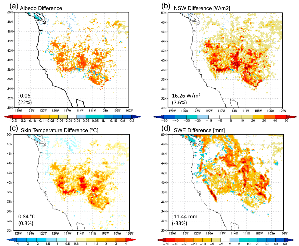
Figure 8. MAM 2009 difference in modeled (a) albedo, (b) net shortwave (NSW) radiation [W/m 2 ], (c) skin temperature [°C], and (d) SWE [mm] between wrf_AER and wrf_NOAER simulations using WRF/SSiB/aer. Statistics listed in each panel refer to area averages during MAM over 30–50°N, 129°W to 102°W, wherever difference for albedo, NSW, skin temperature, and SWE are greater than 0.02, 5 W/m 2 , 0.2°C, and 1 mm, respectively, with the percent change in parentheses.
