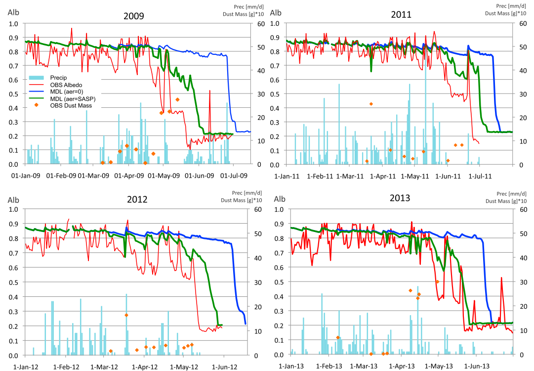
Figure 2. Observed and modeled albedo using SSiB-3/aer for four different years at the SASP site, along with precipitation [mm/day], dust events, and dust mass [g] × 10 (right vertical axis).
