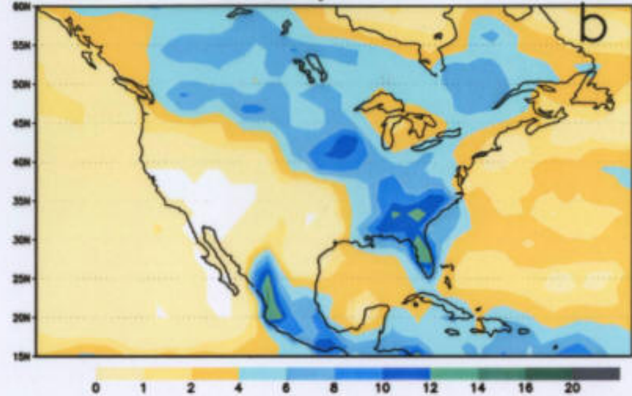
reanalysis data
