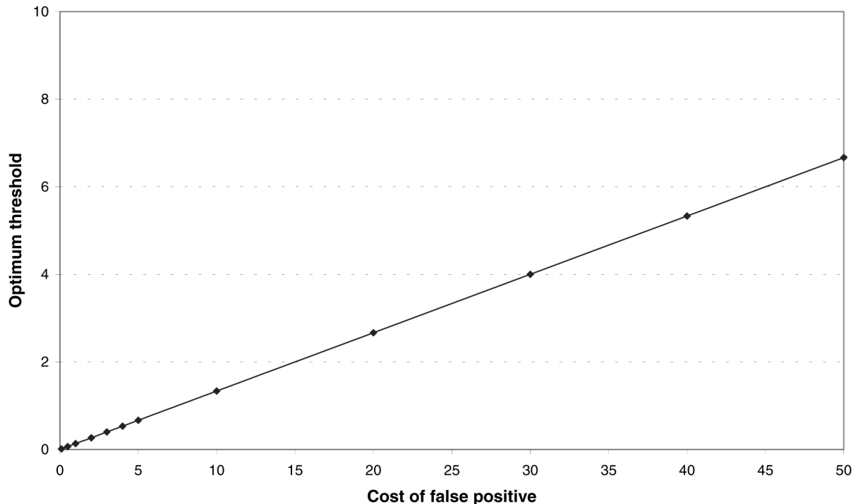
Figure 2. The optimum threshold (likelihood ratio) for adopting a belief S where the cost of the FN is fixed at 5 and the cost of the FP varies, with the probability of s set at 0.6. A threshold greater than 1 represents a bias against adopting S . For explanations see text.
