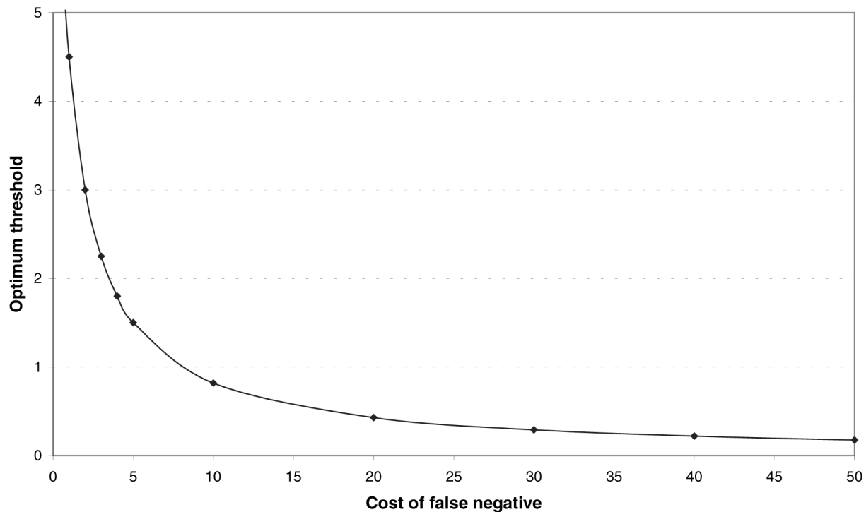
Figure 1. The optimum threshold (likelihood ratio) for adopting a belief S where the cost of the FP is fixed at 1 and the cost of the FN varies, with the probability of s set at 0.1. A threshold less than 1 represents a bias toward adopting S . For explanations see text.
